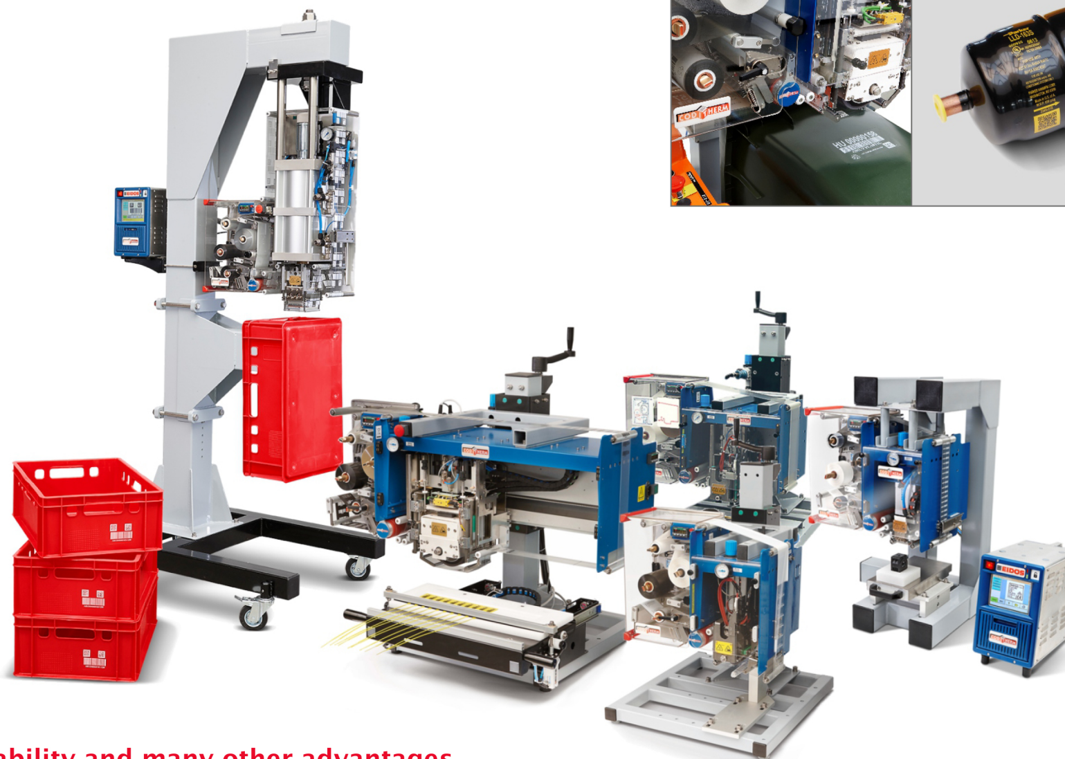
Each version of Coditherm can be mounted on a table-stand or on a floor-stand.
